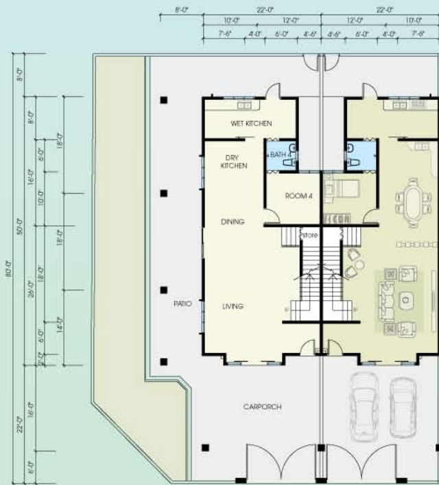
22'x80' • GROUND FLOOR PLAN
